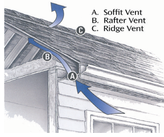
Above, from left rim joist insulation, rafter vent properly positioned and insulated, illustration showing proper attic venting system, and loose fill blown-in insulation in attic rafters.
