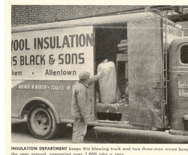
INSULATION DEPARTMENT keeps this blowing truck and two three-man crews busy the year around, averaging over 1,000 jobs a year.
